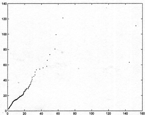
Figure 13: Mean-excess plot of the Danish fire insurance data. The plot looks approximately linear indicating Pareto-like tails.
