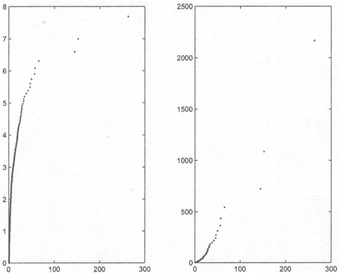
Figure 8: Quantile-quantile plots for the Danish fire insurance claims. Left: qq-plot with exponential reference distribution. The plot curves down which indicates that data has tails heavier than exponential. Right: qq-plot against a Pareto(1) distribution. The plot is approximately linear which indicates that the data may have a Pareto( \alpha ) distribution with \alpha close to one.
