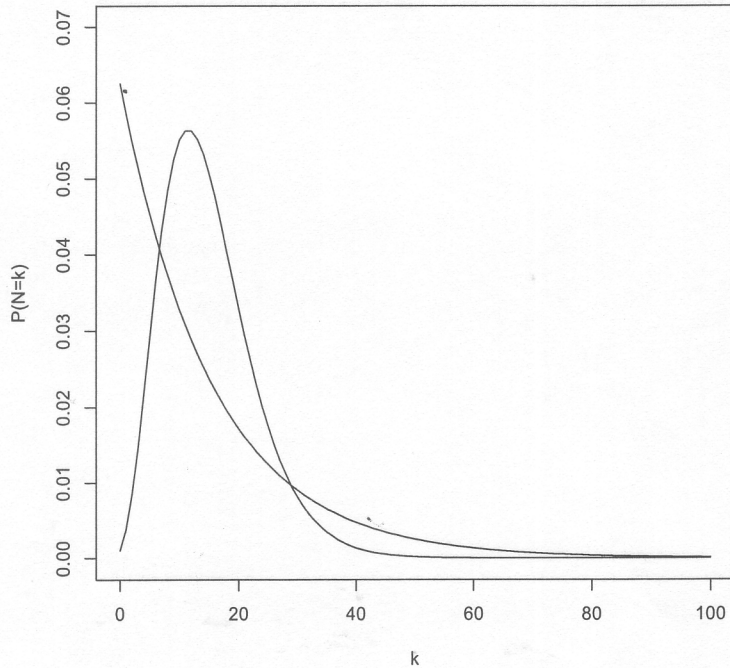
Figure 33: P(N = k) for k = 0, \dots, 100 for m = 1 and m = 5 . For m = 1 the probability P(N = k) is decreasing in k , for m = 5 the probability P(N = k) first increasing in k and then decreasing.
