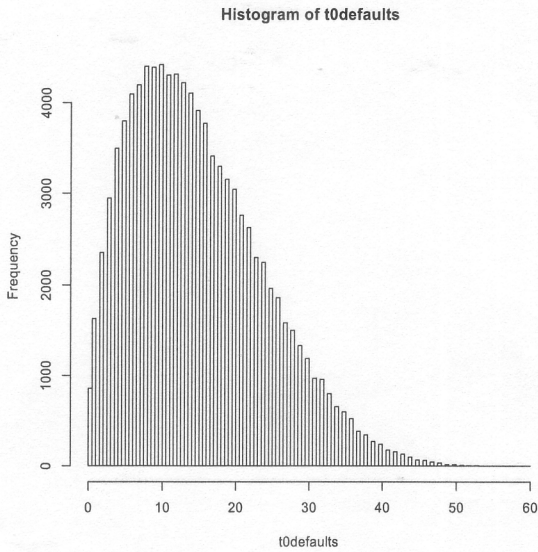
Figure 31: Histograms of the number of defaults: (a) Gaussian copula (upper) and (b) t_4 copula (lower).
