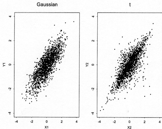
Figure 27: Samples from two distributions with standard normal margins, R_{12} = 0.8 but different dependence structures. (X1, Y1)^T has a Gaussian copula and (X2, Y2)^T has a t_2 -copula.
