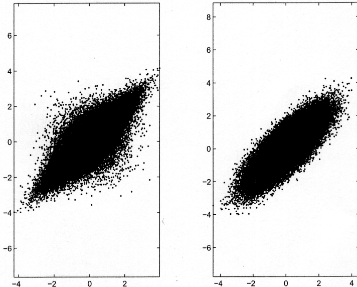
Figure 21: Illustration of two bivariate distributions with linear correlation \rho_L = 0.8 and standard normal marginal distributions. The one to the left has tail dependence \lambda_u = \lambda_l = 0.49 and the one to the right has \lambda_u = \lambda_l = 0 .
