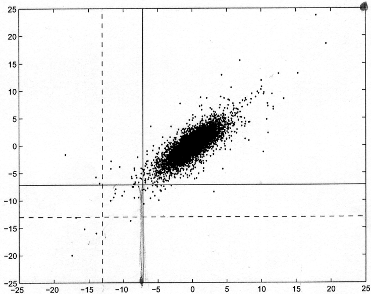
Figure 20: Illustration of lower tail dependence.
