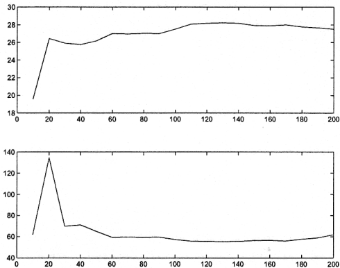
Figure 16: Up: The estimated 99% quantile as a function of N_u . Below: Estimated values of 99% Expected Shortfall as a function of N_u .
