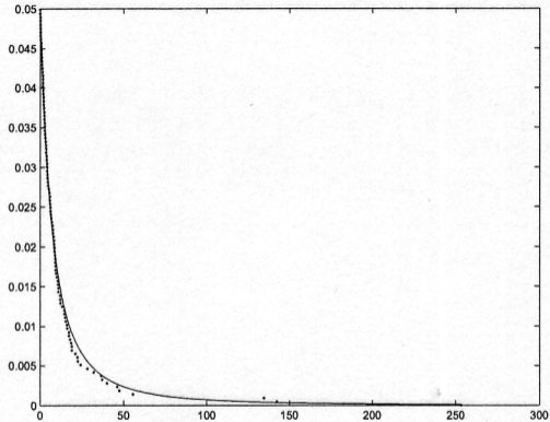
Figure 15: The empirical tail of the Danish data and the fitted approximation using POT.
