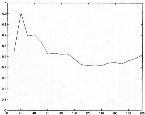
Figure 14: Maximum likelihood estimates of \gamma as a function of the number of exceedances N_u . It shows a rather stable behavior for N_u in the suggested region (39, 109).
