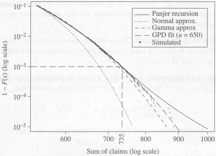
Figure 10.5. Simulated CPoi(100, LN(1, 1)) data ( n = 100\,000 ) with normal-, translated-gamma, GPD and Panjer recursion (see Example 10.17) approximations (on log-log scale).
