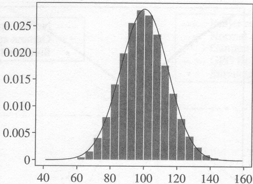
Figure 10.3. Histogram of simulated compound loss data ( n = 100\,000 ) for S_N \sim \text{CPoi}(100, \text{Exp}(1)) together with normal approximation (10.14).
